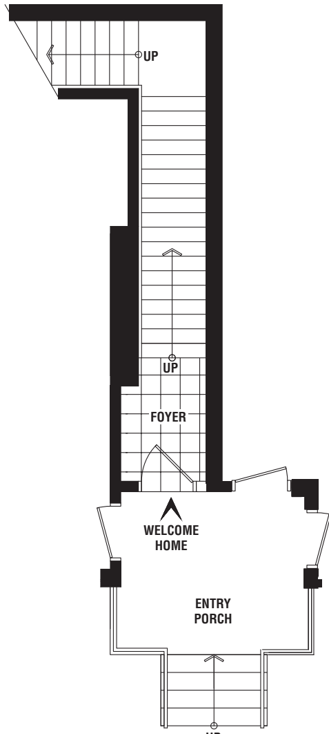
ENTRY LEVEL
