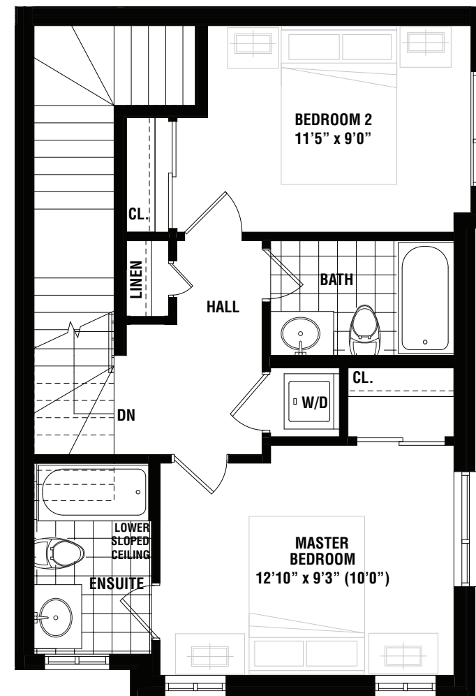
UPPER LEVEL
