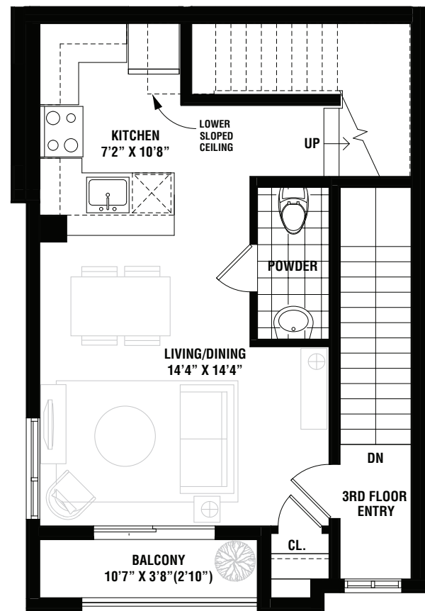
MAIN LEVEL
